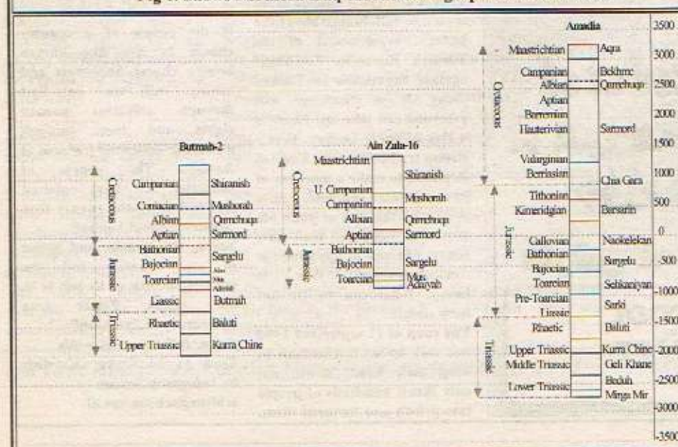
Fig 1. Shows Northern Iraq chrono-stratigraphical successions.
