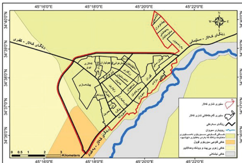
GEOLOGICAL MAP OF QARADAGH – KALAR BASIN, Produced by FAO ,Northern Iraq ,Coordination Office, Scale 1 : 50000 .
